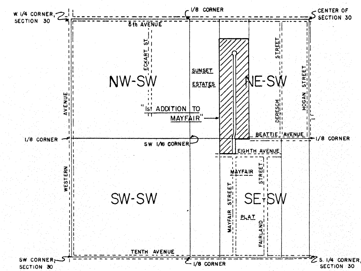
-LOCATION SKETCH- PLAT IS LOCATED IN THE E. 1/2 SW 1/4, SECT. 30, T31N, R11E CITY OF ANTIGO, LANGLADE COUNTY, WISCONSIN
